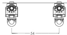
A13-SF200/100S | small wheeled wave fold carrier
